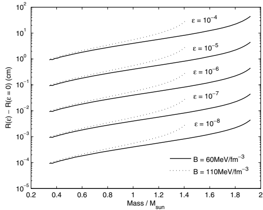
Figure 1. The difference R(\epsilon \neq 0) - R(\epsilon = 0) in stellar radius as a function of stellar mass. Solid lines are for bag constant B = 60 \text{ MeV fm}^{-3} , and dotted lines for B = 110 \text{ MeV fm}^{-3} . The quantity \epsilon is defined by introducing P_{\perp} = (1 + \epsilon)P , where P_{\perp} and P are the radial and tangential pressures, respectively.
